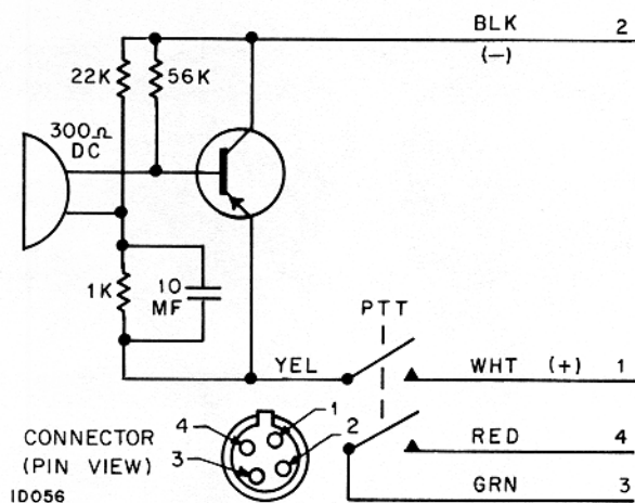
Figure 2. Amplifier Circuit
