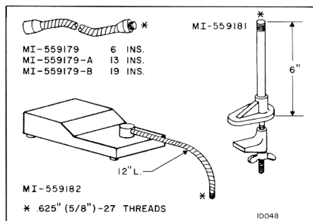
Figure 7. Desk Microphone Supports
