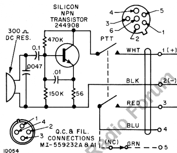
Figure 3. Amplifier Circuit
