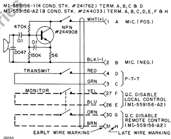
Figure 5. Amplifier Circuit
