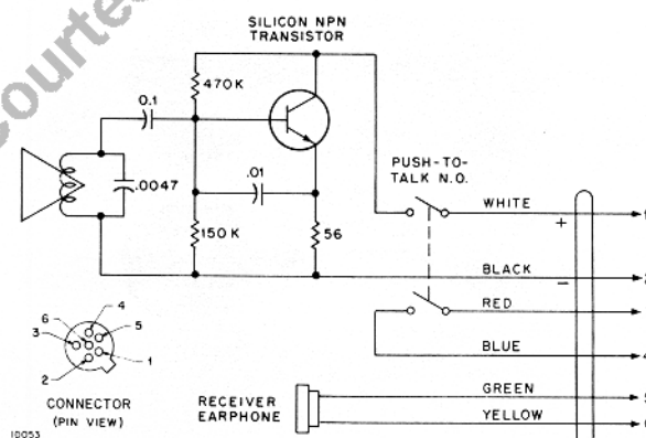
Figure 6. Amplifier Circuit
